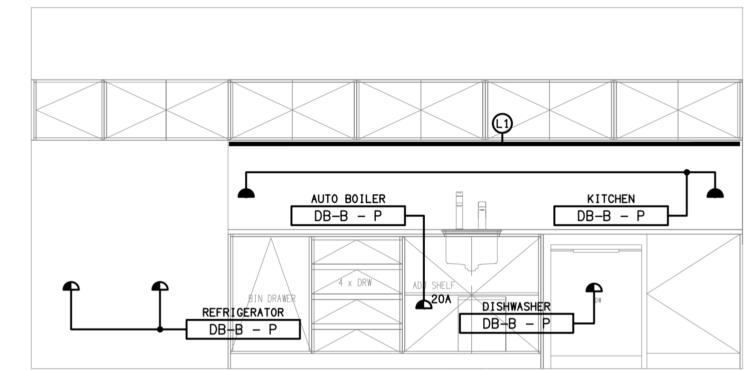
DETAIL A LUNCH ROOM KITCHENETTE ELEVATION SCALE 1: 25
